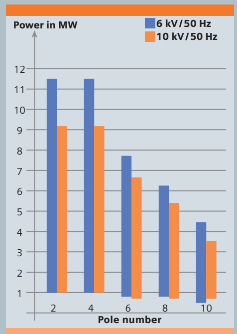
1RA4/1RN4/1RN6/1RP6 series
