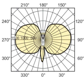
Light Distribution Diagram - MASTERC CDM-T 150W/830 G12 1CT
