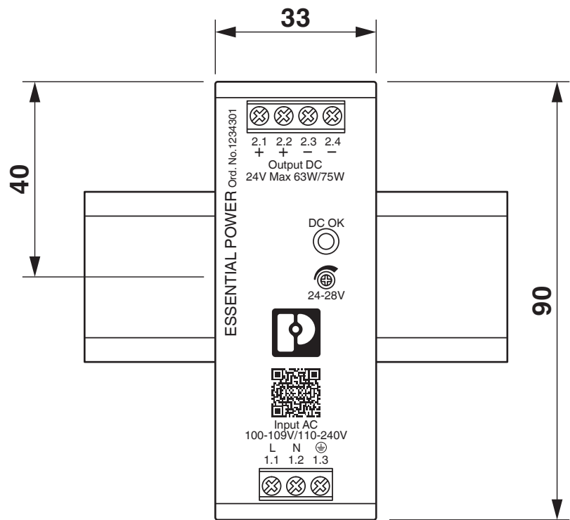
Dimensional drawing
