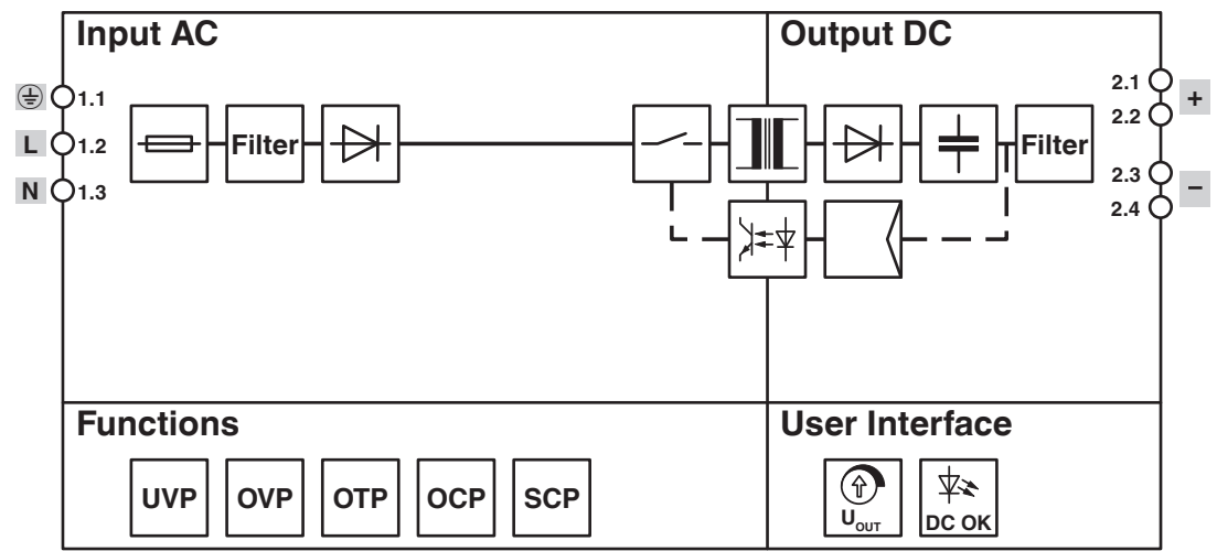
Block diagram
