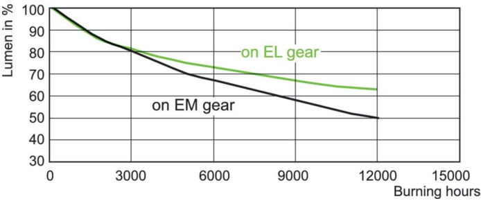
Lumen Maintenance Diagram - MASTERC CDM-T 70W/942 G12 1CT/12
