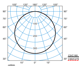
Siella G8 M73 DW 28-40/3ML-8MC ET (stage 2)
