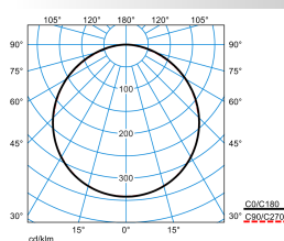
Siella G8 M73 DW 28-40/3ML-8MC ET (stage 1)
