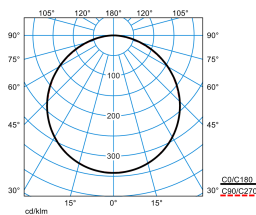
Siella G8 M73 DW 28-40/3ML-8MC ET (stage 5)
