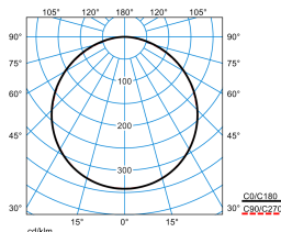
Siella G8 M73 DW 28-40/3ML-8MC ET (stage 6)
