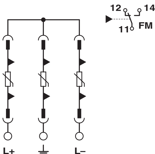
Circuit diagram
